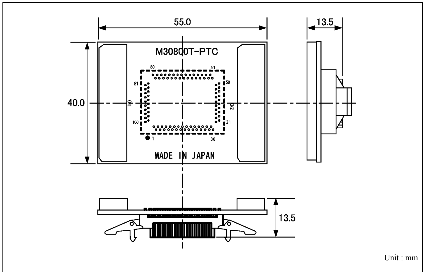
Figure 4.4 External dimensions of the M30800T-PTC
